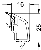
Glasleiste 16/25 Glazing bead 16/25 19584...
