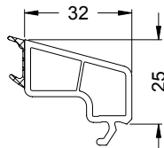
Glasleiste 32/25 Glazing bead 32/25 19562...
